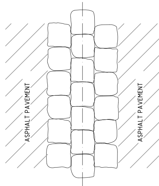
DETAIL 3: THREE ROW PITCHER CHANNEL SETTING DETAIL
