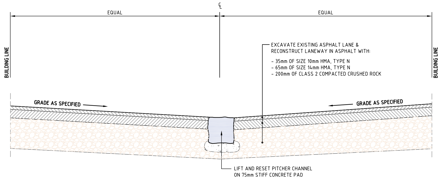
DETAIL 1: ASPHALT LANEWAY PAVEMENT RECONSTRUCTION
