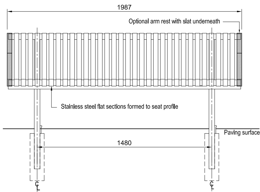
Elevation (Front)
