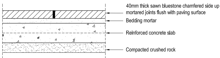
Typical section
