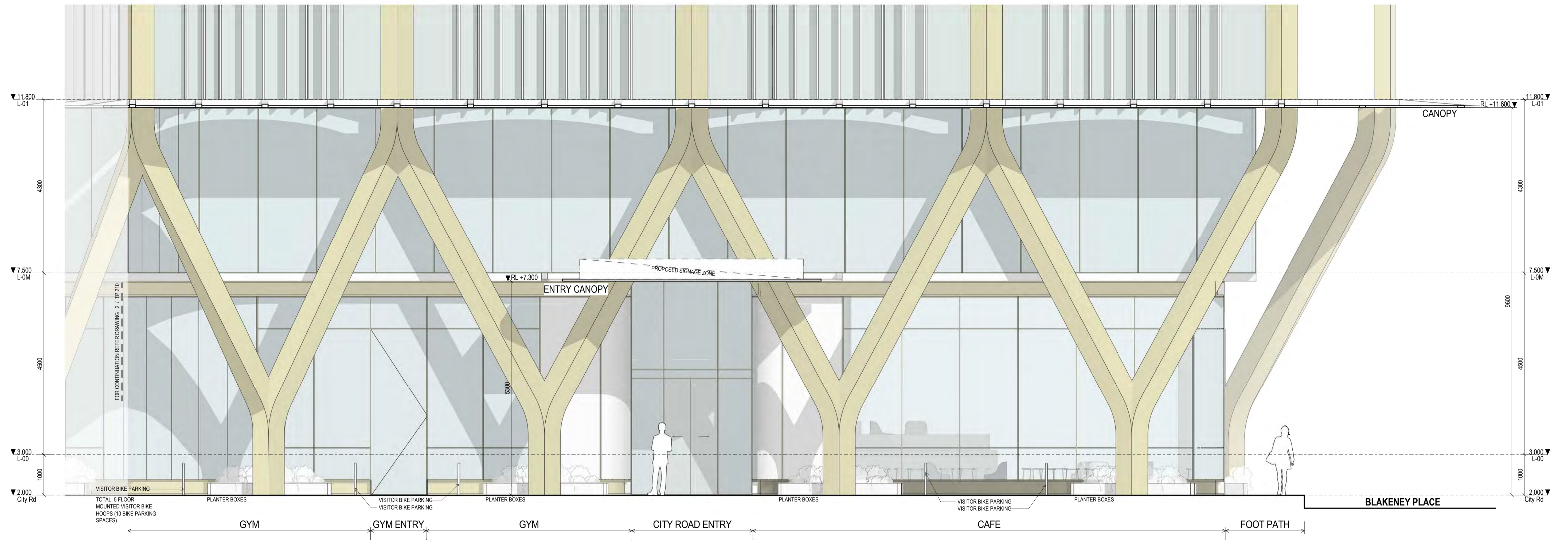
1 STREET ELEVATION - EAST TP.201 1:50
