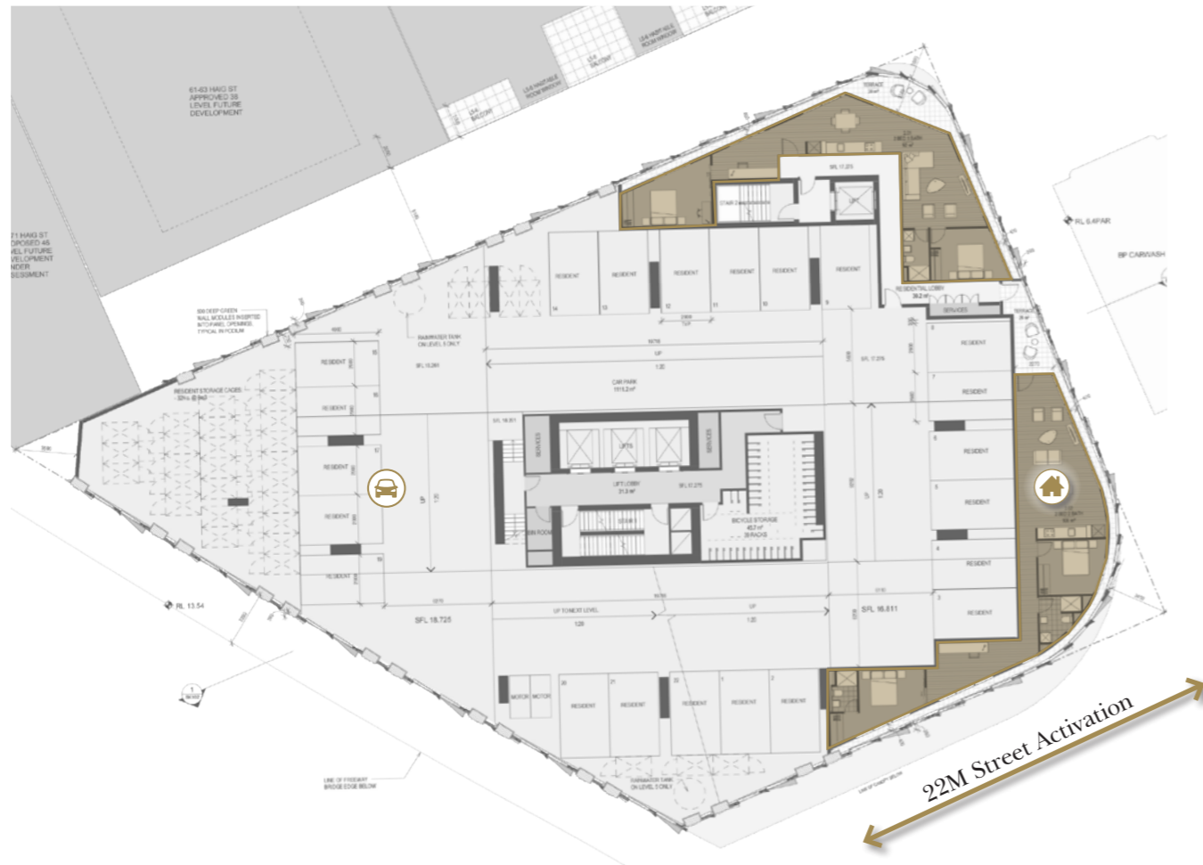
Existing Plan
