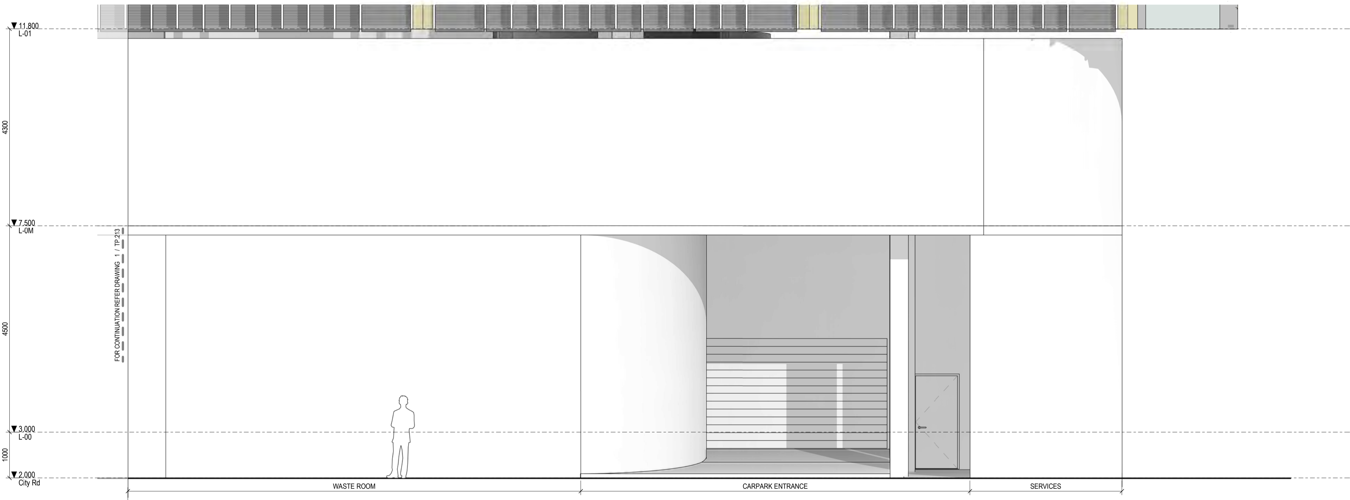
2 STREET ELEVATION - WEST - PART B TP.203 1:50
