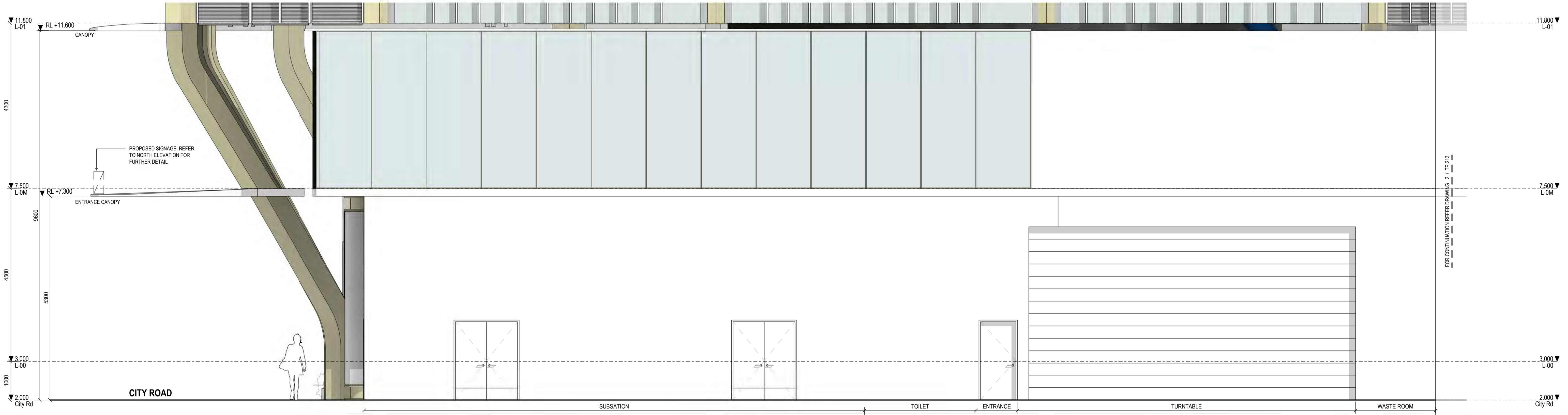
1 STREET ELEVATION - WEST - PART A TP.203 1:50
