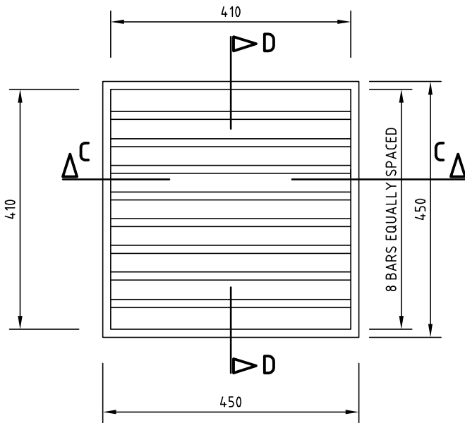
PLAN OF GRATING
