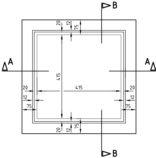
PLAN OF FRAME
