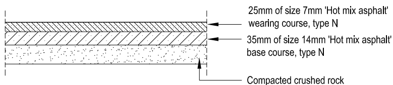
Standard 60mm thick asphalt footpath for outside the Central City area (Suitable for areas of the municipality outside of the Central City & Docklands or as approved)
