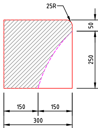
CROSS SECTION
