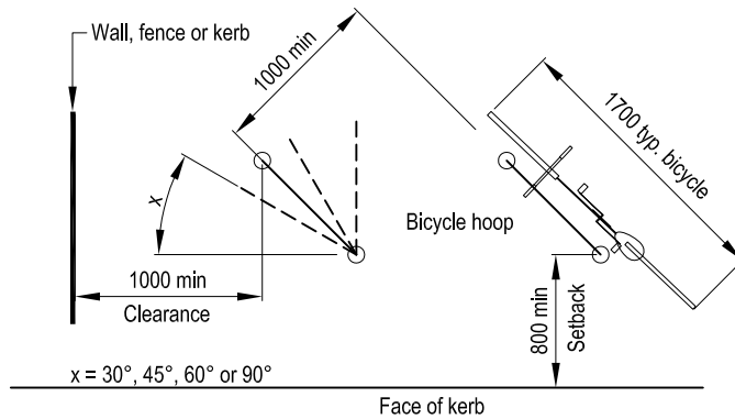
Plan Bike hoops angled to kerb
