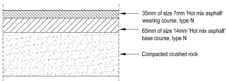
Standard 100mm thick asphalt road pavement on crushed rock base (Suitable for all areas of the municipality or as approved)
